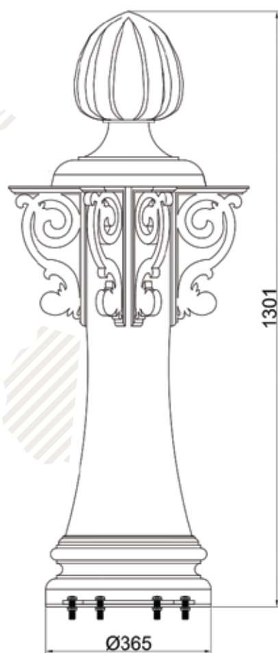
Front View All Dimension In MM
