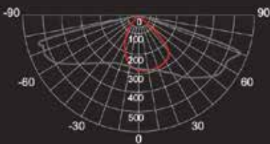
BATWING LIGHT DISTRIBUTION CURVE
